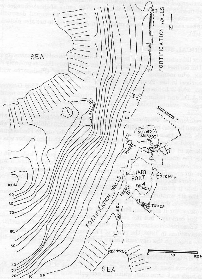
Figure 2. Plan of Phalasarna harbor. Location of trenches A, B and C are shown.
