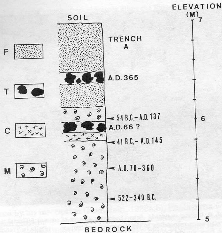
Figure 6. Simplified stratigraphy of trench A. F: freshwater (terrestrial) deposits; T: tsunami deposits; C: confined marine deposits; M: marine deposits. Arrows with dates correspond to the positions of four samples for which new radiocarbon dates were obtained from the present survey (see Table II).
