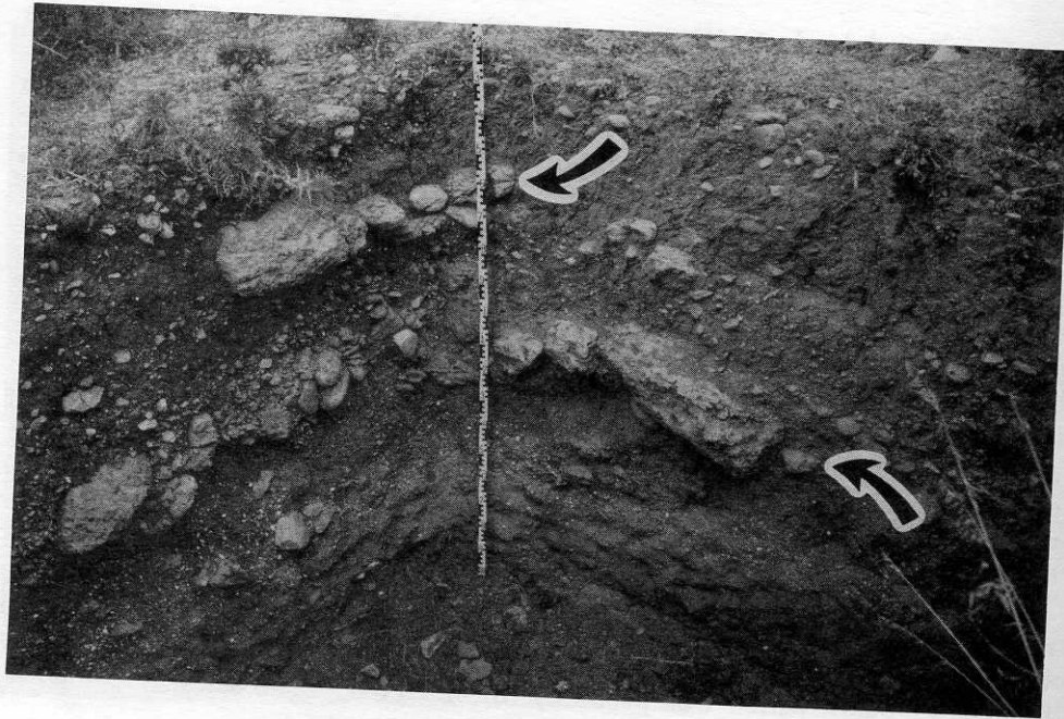
Figure 4. Trench A, in the middle of the military port basin. Arrows indicate two horizontal layers of coarser material with blocks, interpreted as tsunami deposits (photo by P. A. Pirazzoli).
