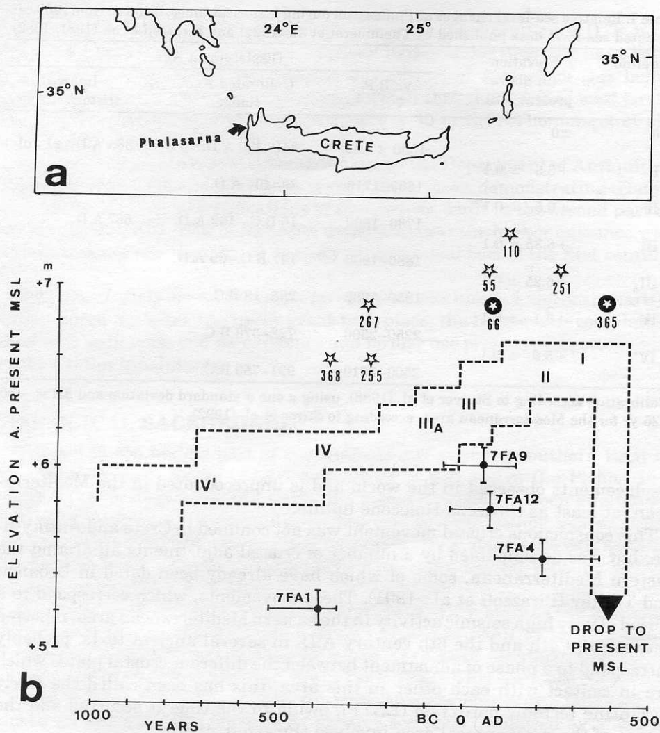
Figure 1. (a) Location of Phalasarna harbor. (b) Band of relative sea-level changes at Phalasarna between 1000 B.C. and A.D. 500, compared with historically destructive earthquakes (open stars) and tsunamis (encircled stars) in Crete. The radiocarbon dates plotted in the graph refer to four samples mentioned in the text.
