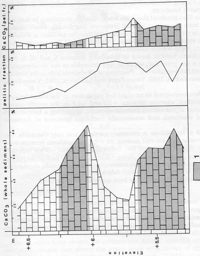
Figure 5. Carbonate and pelitic contents of the whole sediment and carbonate content of the pelitic fraction (pelitic fraction is designated as <40 \mu\text{m} ) along a vertical profile in Trench A. The carbonate fraction results from the association of marine biogenic particles and pedogenetic remains; in each case (whole sediment or pelitic fraction), it decreases above +6 m with the decline of marine intrusion; concurrently, the pelitic fraction is replaced by the sandy quartzos fraction. Note a recurrence of marine influences towards +6 m. 1: dominant marine biogenic particles.
